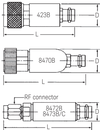
Figure 5. Drawing dimensions given in specification table
